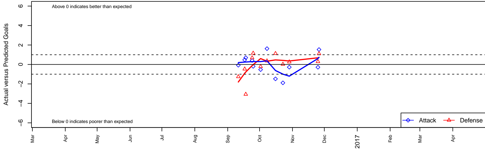
San Diego SC Academy Navy G01 Dots are actual minus expected GF (blue circles) and GA (red triangles). Blue line is smoothed change in attack strength. Red is smoothed change in defense strength.
